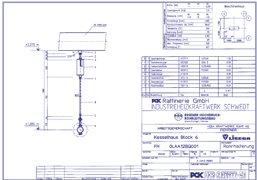
CAD drawing according to customer requirements
