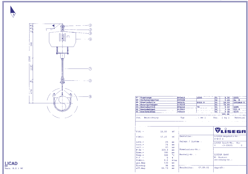
LICAD drawing
